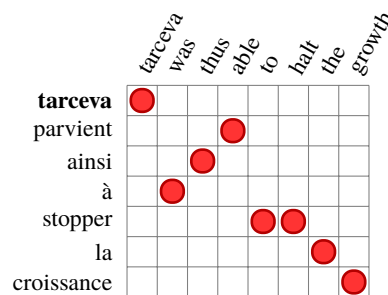
Figure 3: User translation word alignment obtained via prefix decoding and dynamic phrase table augmentation.
